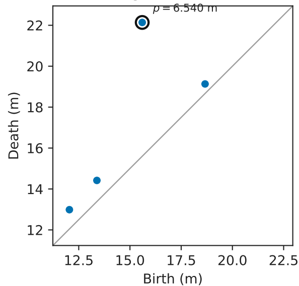
(a) Individual diagram ( \delta = 2.75 m, frame 95)
